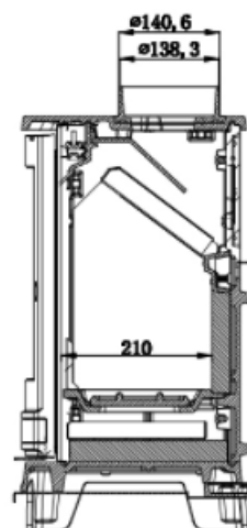
CUT VIEW A-A
