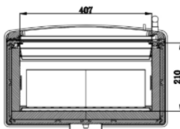
CUT VIEW B-B
